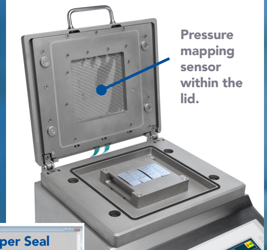
FIGURE 5 THE BONFIGLIOLI PILL PACK MACHINE INCLUDES A PRESSURE MAPPING FEATURE THAT IDENTIFIES LEAKS IN PILL PACKS
