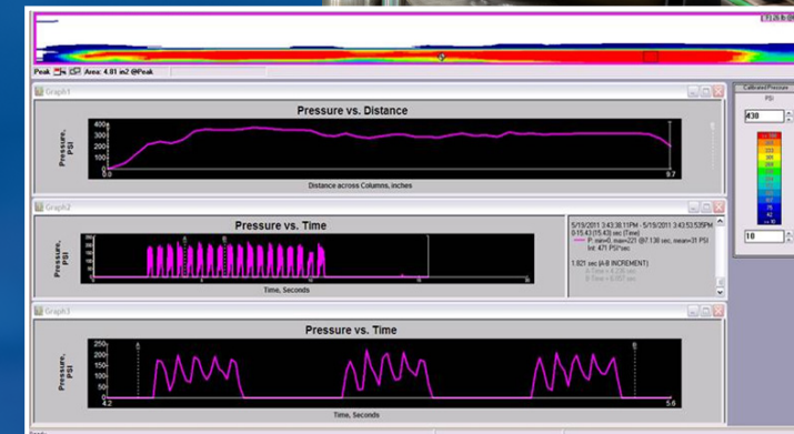
FIGURE 4 PRESSURE MAPPING OUTPUT OF IMPACTS AS BOTTLES AND CONTAINERS ADVANCE THROUGH A FILL LINE OPERATION
